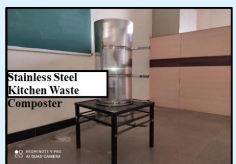
Design and Development of Composter for Kitchen Waste
